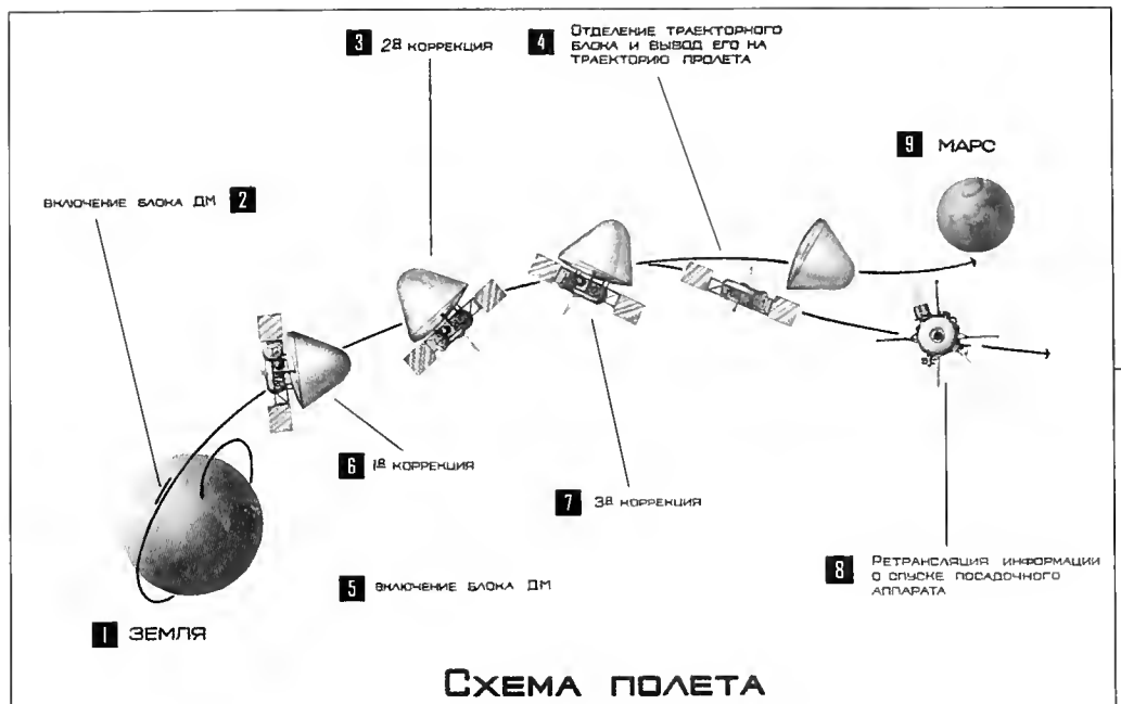
Figure 24. The Flight Profile of the 5M Spacecraft— (1) Earth, (2) activation of block DM, (3) second correction of reactive block and its injection into flyby trajectory, (5) insertion of the DM block, (6) first correction, (7) third correction, (8) retransmission of the information on the lander descent, and (9) Mars
